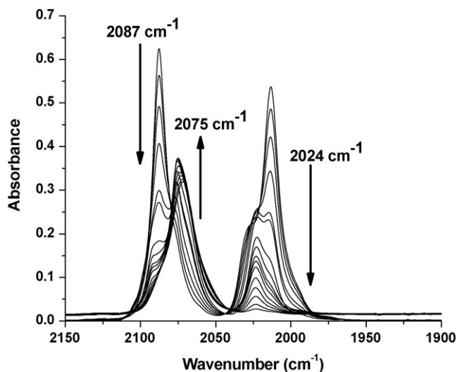
Fig. 1. Series of IR spectra \{\nu(\text{CO}) \text{ region}\} illustrating the reaction of 1a with MeI at 25 °C.
